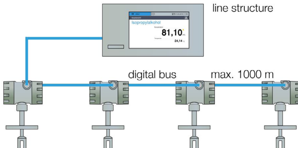
Controller with connection of up to four sensors
