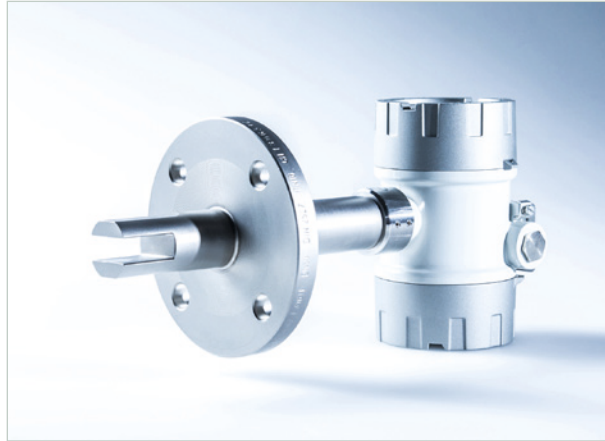
Tauchsensormodell Ex 40-40
